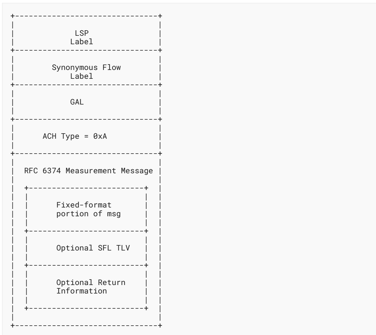
Figure 5: RFC 6734 Query Packet with SFL
