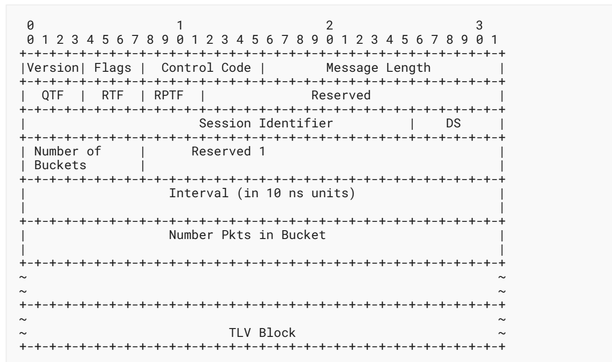
Figure 2: Time Bucket Jitter Measurement Message Format
